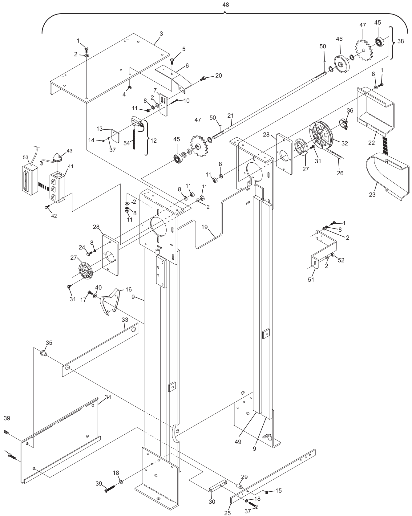
Elevator Assembly - Round Frame Hole Short Pit Machines Series 43 and Above
