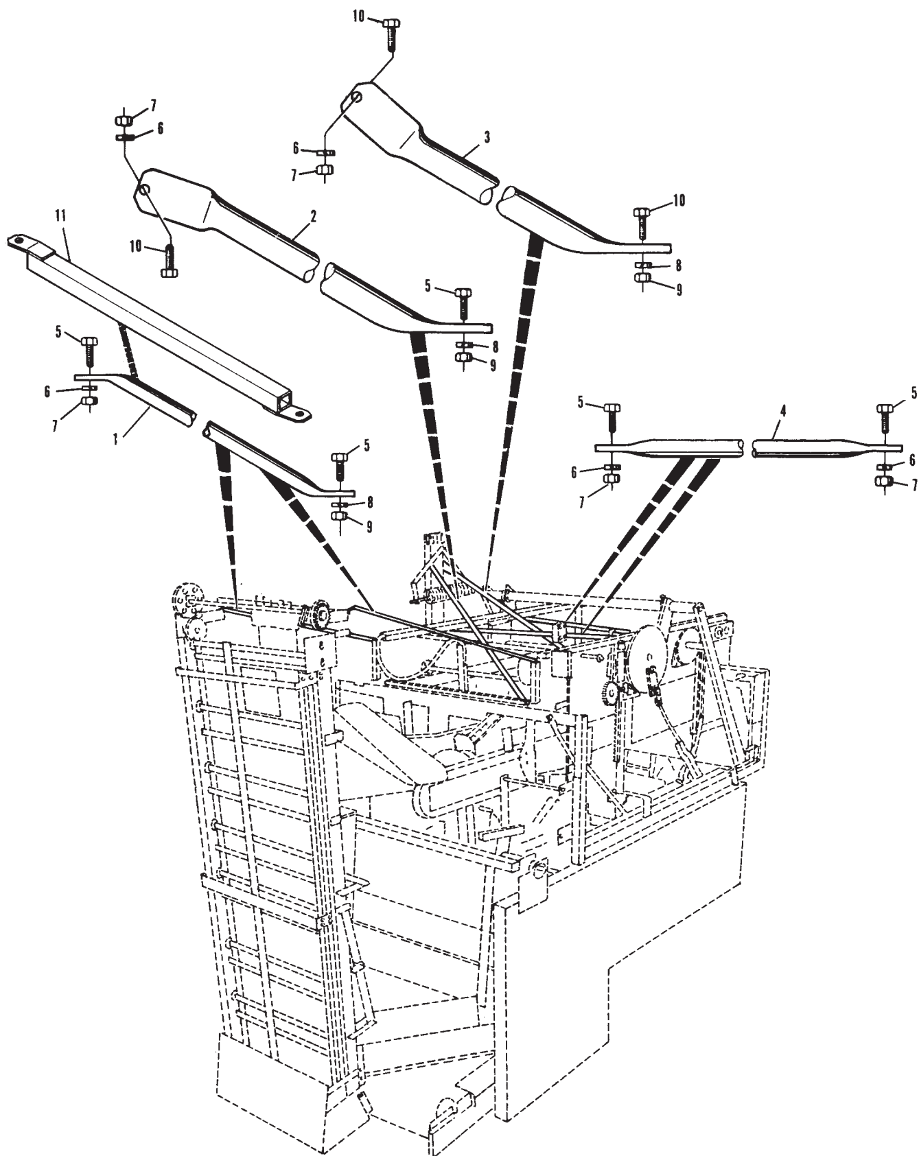
Support Braces
