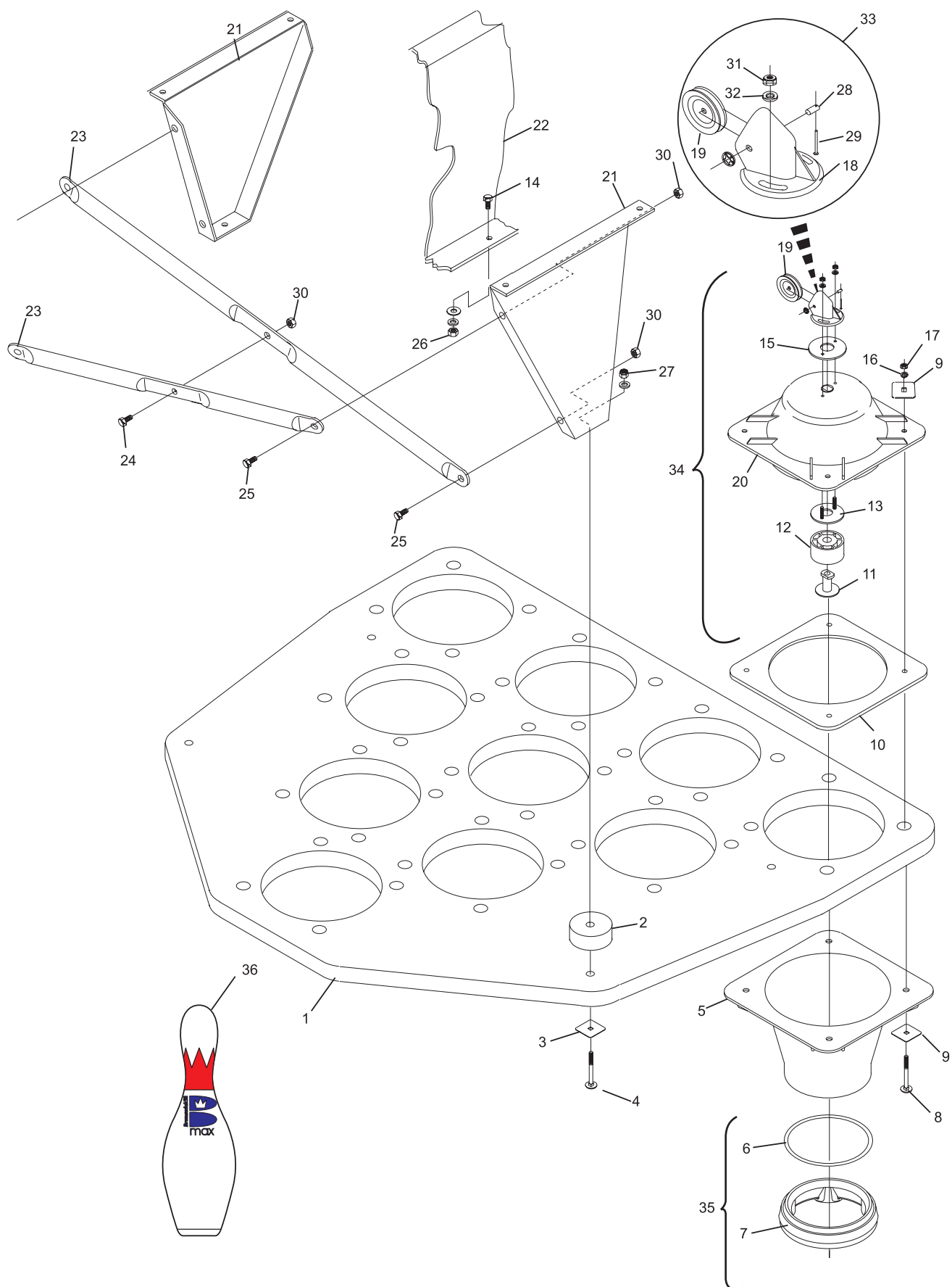
Setting Platform Assembly
