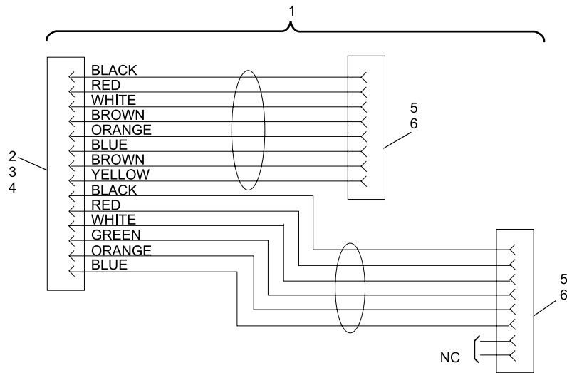
GAMESETTER POWER & PERIPHERAL CONTROL CABLE ASSEMBLY
