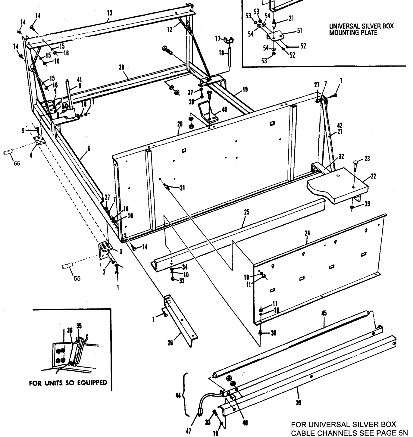
Frame Assembly (GS-96 and Below)
