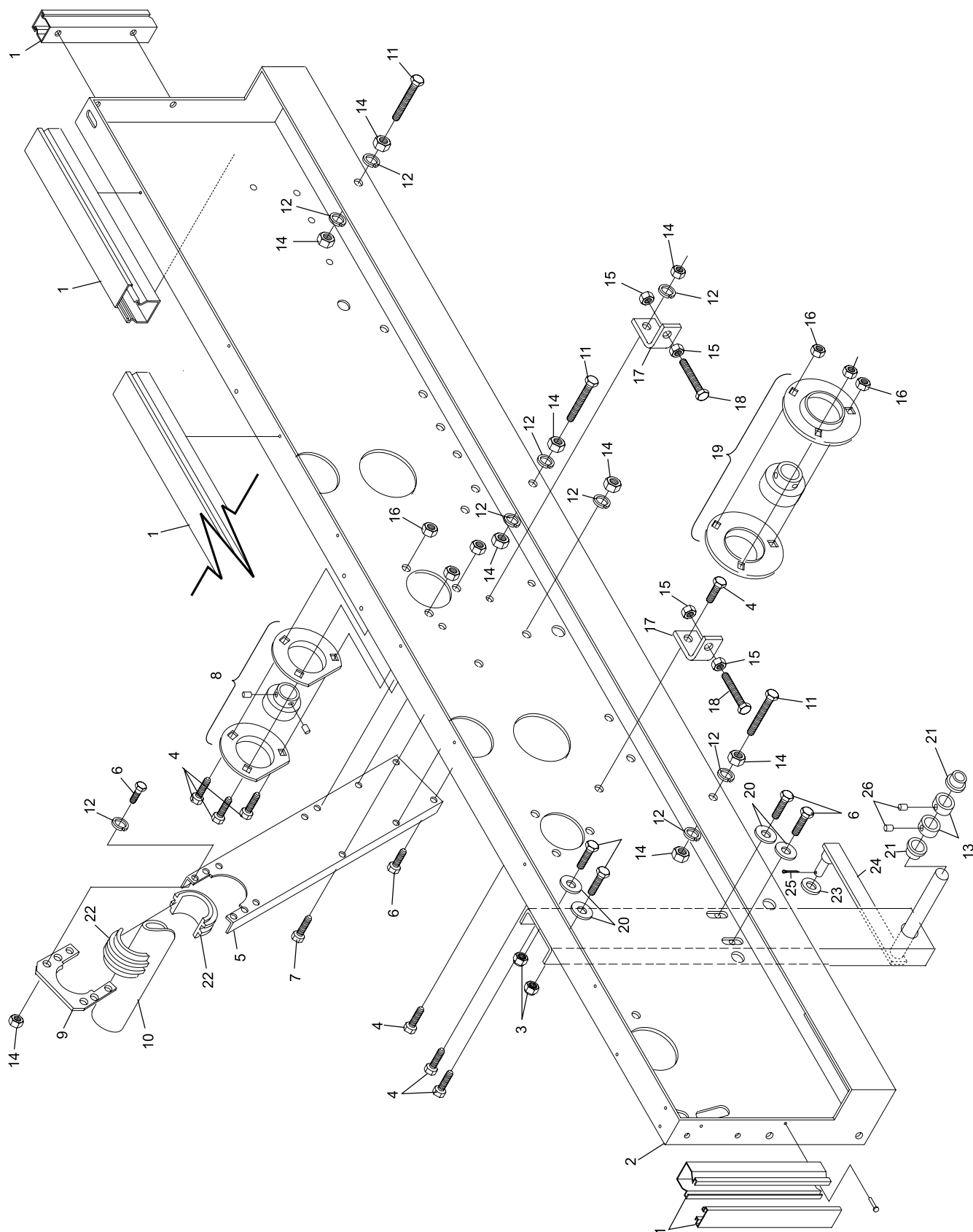
Left Drive Frame Assembly (Machine Series 443 and Above)
