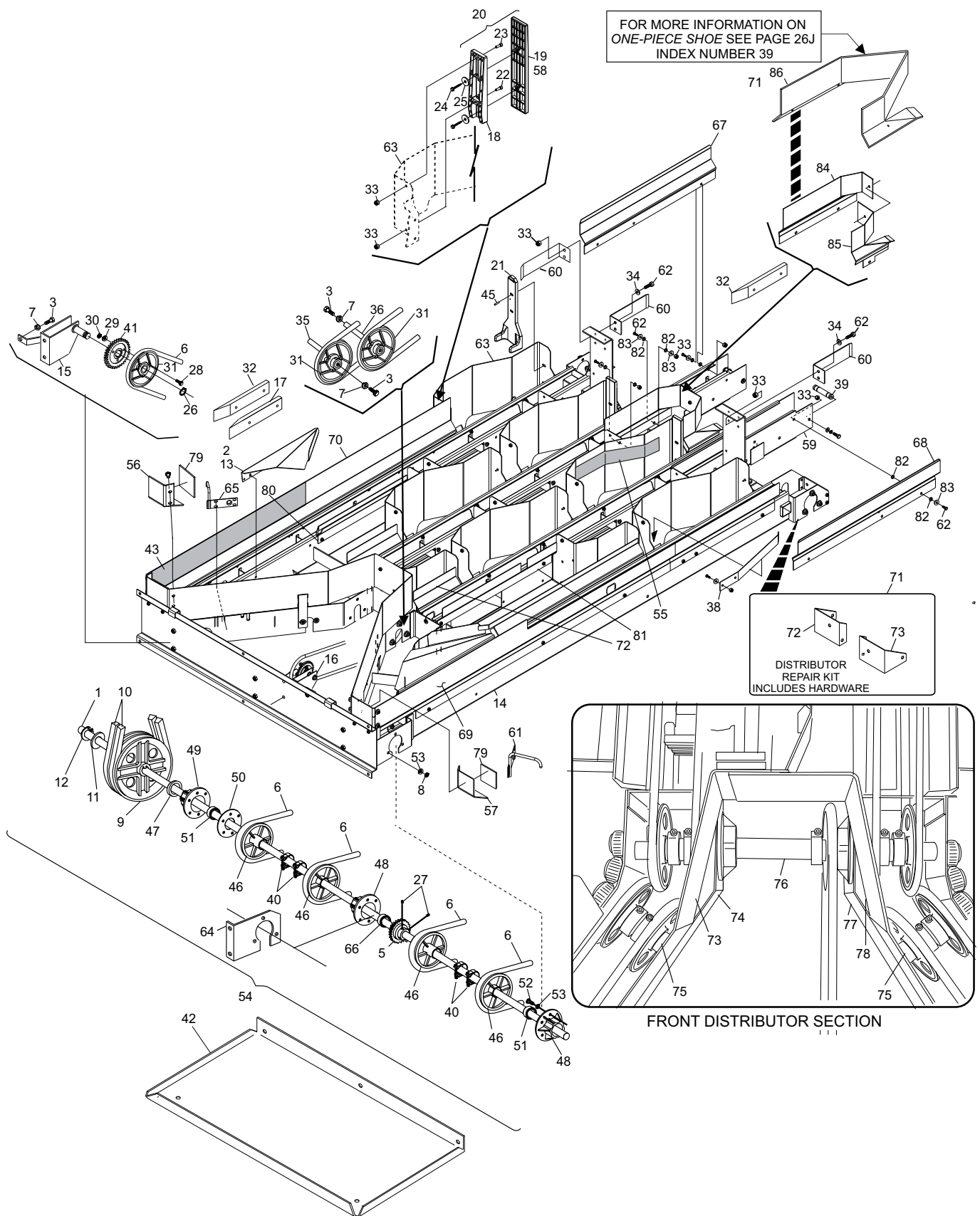
Dual Feed Distributor
