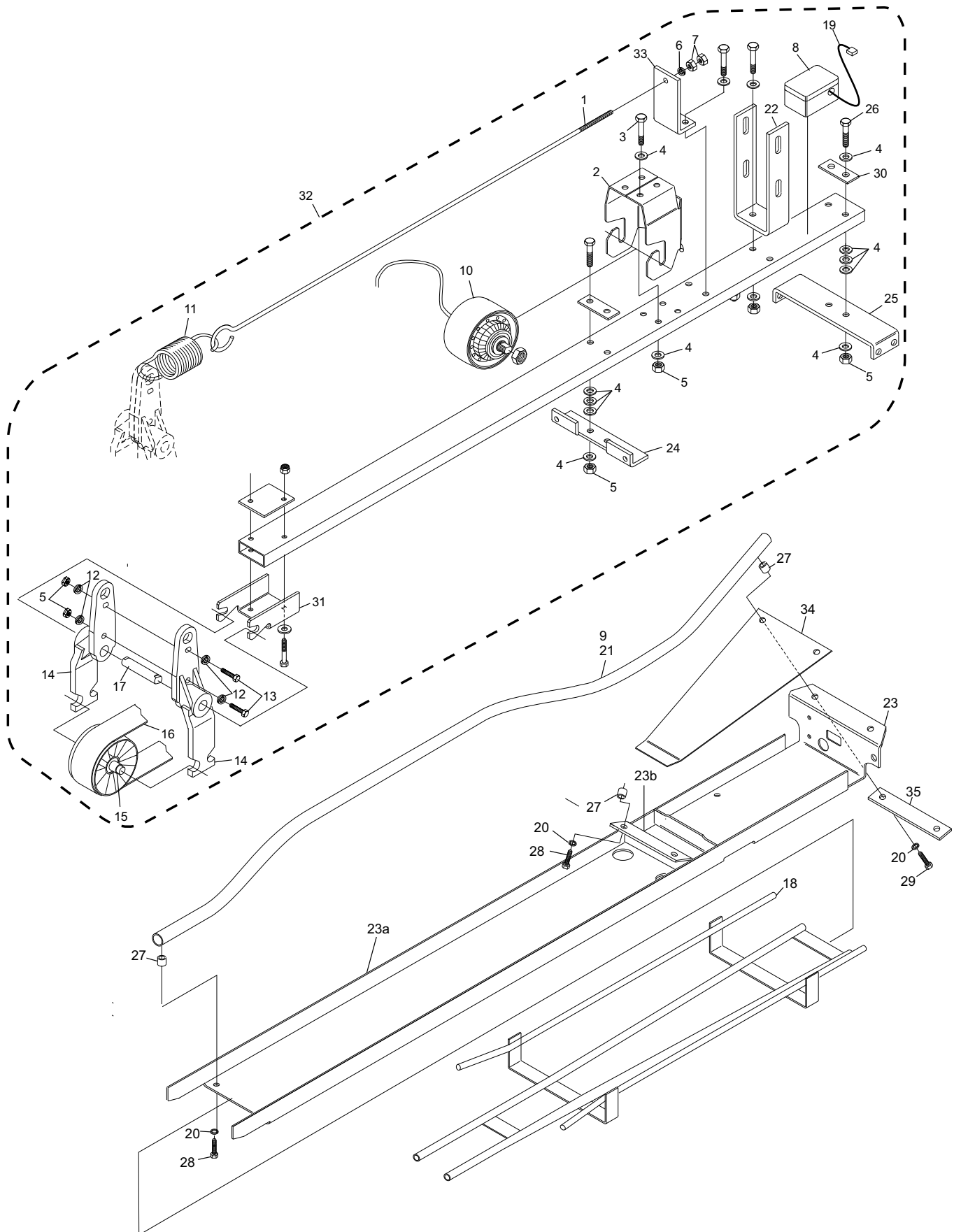
GS-X/CPO Ball Accelerator
