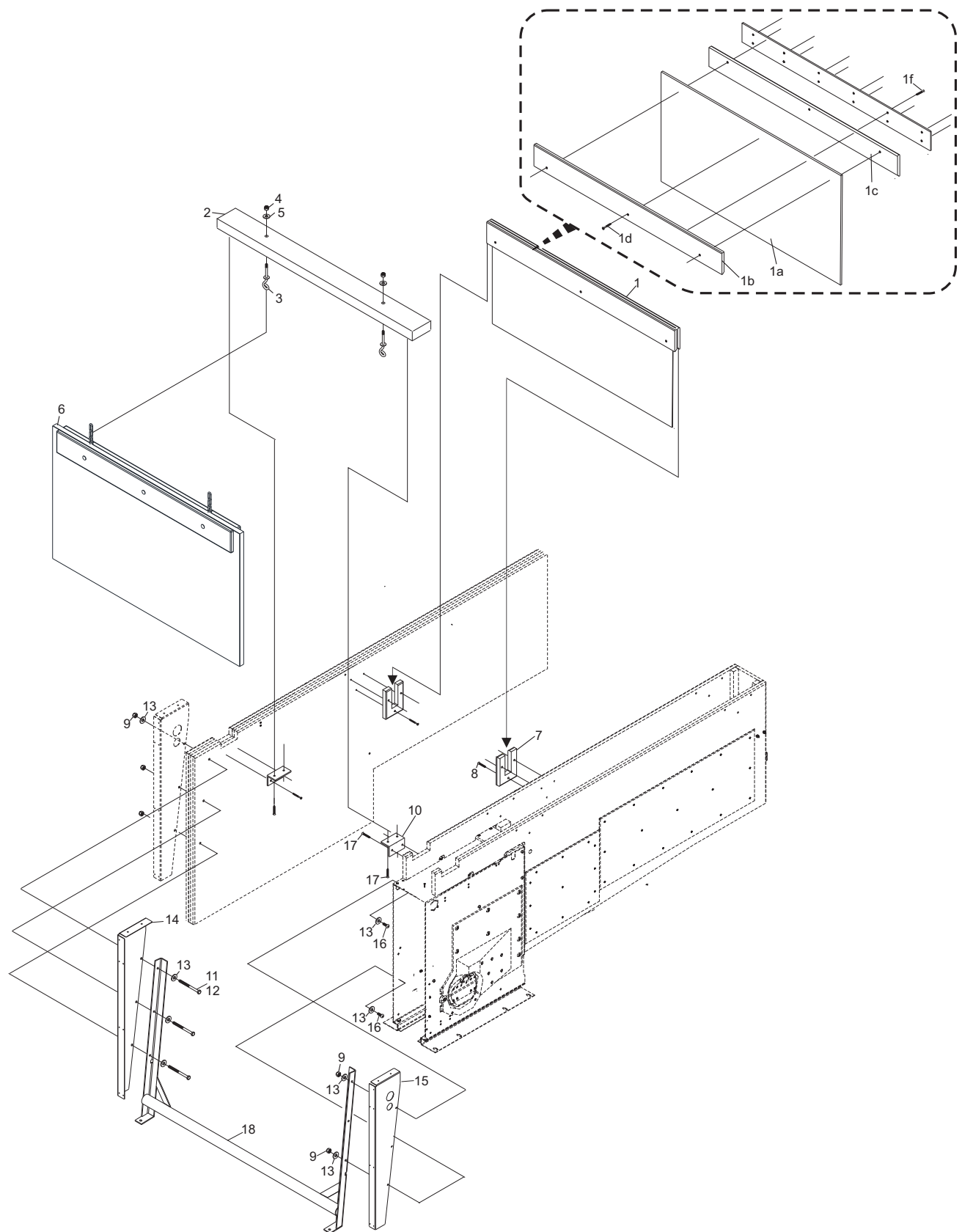
Ball Cushion/Pit Curtain
