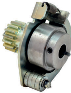
AV 610-704-006D Duraclutch Asm • The original brake clutch • Positive drive action • Developed in the UK
