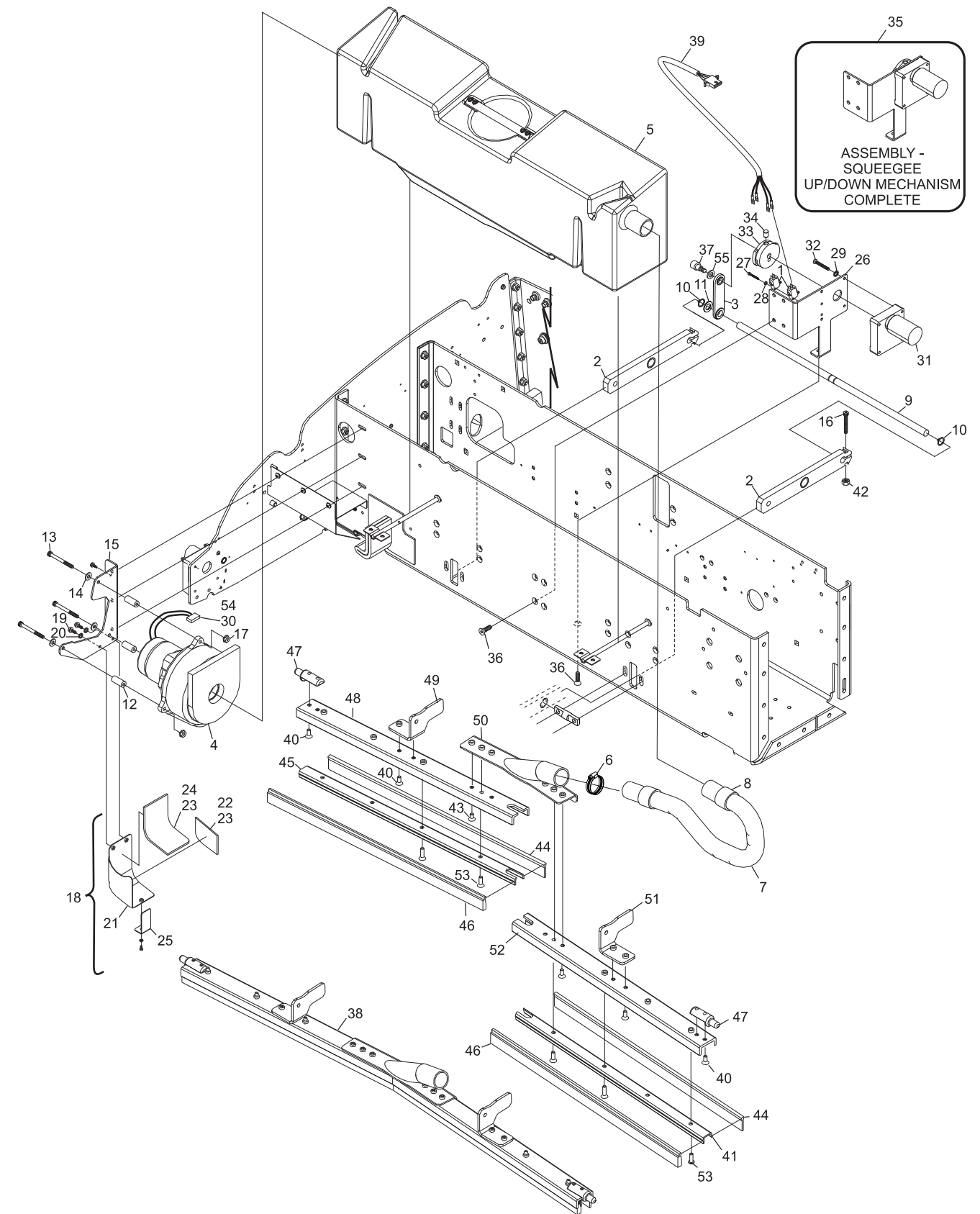
Squeegee & Waste System
