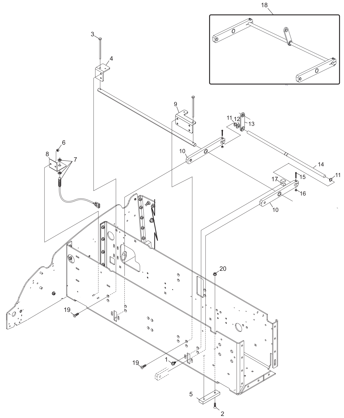
Squeegee Linkage System
