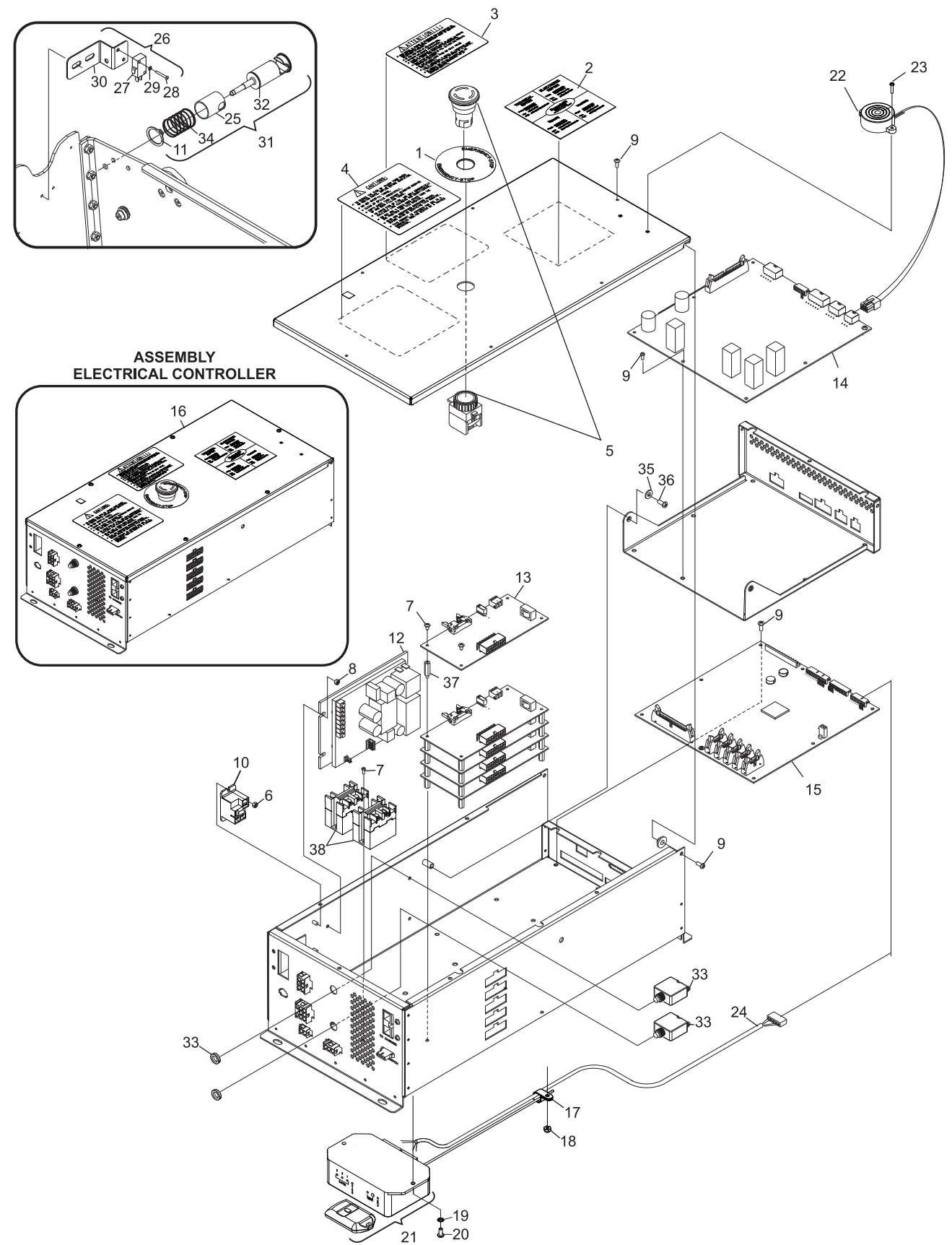
Electrical Enclosure
