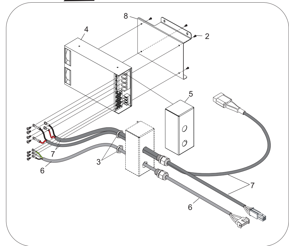
AC/DC Power
